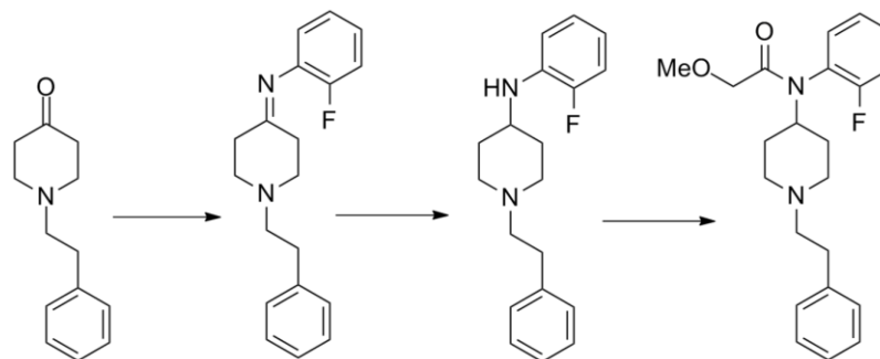
Figure 1: Ocfentanil synthesis (Huang et al., 1986)
