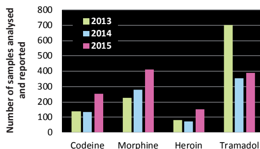
FIG. 17 Trends in the non-medical use of pharmaceutical opioids and heroin among persons in treatment in the United Arab Emirates, 2013–2015
