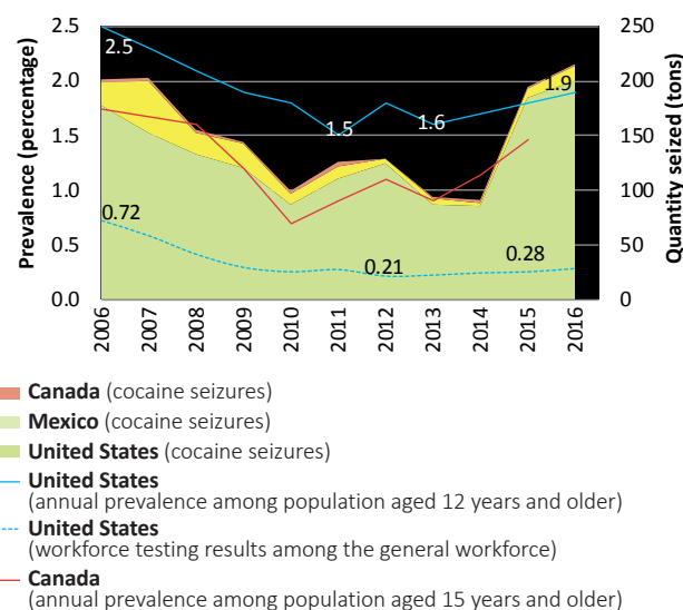
FIG. 5 Seizures of cocaine in North America and annual prevalence of cocaine use in the United States and Canada, 2006–2016
