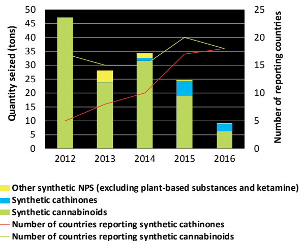
FIG. 7 | Annual quantities of synthetic new psychoactive substances (excluding ketamine) seized globally and number of countries reporting seizures of synthetic cannabinoids or cathinones, 2012–2016
