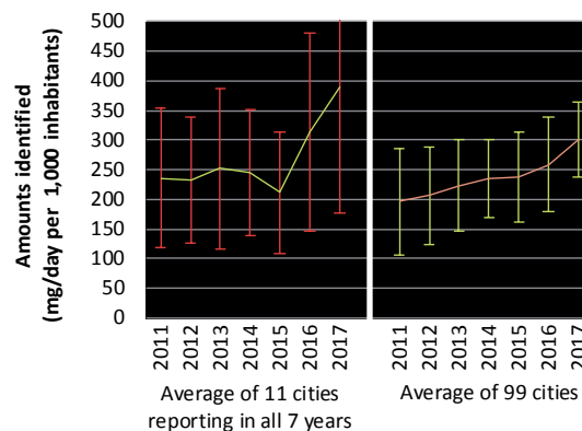
FIG. 7 Benzoyllecgonine found in wastewater per 1,000 inhabitants in Europe (based on data from 99 European cities), 2011–2017
